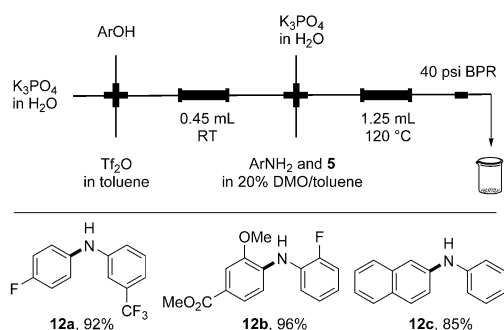
Scheme 1. Two-step flow conversion of phenols into biarylamines via either aryl triflates or tosylates. Yields of the isolated products are reported (average of 2 runs, approximately 1–4 mmol collected). See the Supporting Information for details. Tf = trifluoromethanesulfonyl.
